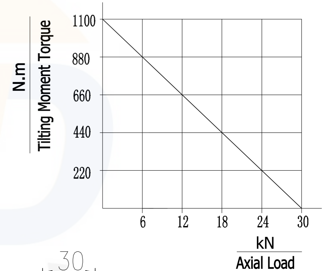
MOMENT LOAD CHART Axial Load & Tilting Moment
